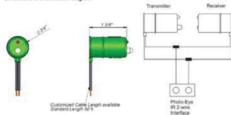
Dimensions and connection diagram
